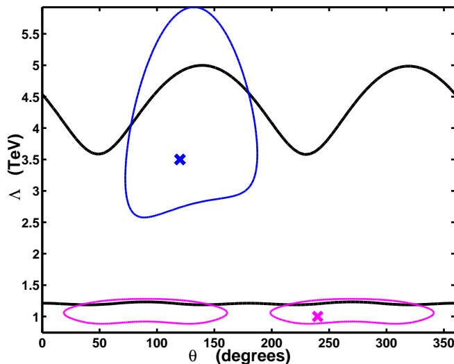
Figure 2: (DARK LINES) 95% confidence level sensitivity of NuSOng to new heavy physics described by Eq. (1) when \nu_\alpha = \nu_\mu (higher curve) and \nu_\alpha \neq \nu_\mu (lower curve). (CLOSED CONTOURS) NuSOng measurement of \Lambda and \theta , at the 95% level, assuming \nu_\alpha = \nu_\mu , \Lambda = 3.5 TeV and \theta = 2\pi/3 (higher, solid contour) and \nu_\alpha \neq \nu_\mu , \Lambda = 1 TeV and \theta = 4\pi/3 (lower, dashed contour). Note that in the pseudoelastic scattering case ( \nu_\alpha \neq \nu_\mu ) \theta and \pi + \theta are physically indistinguishable. From [2].
