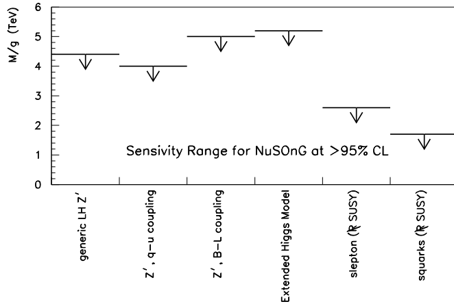
Figure 3: Some examples of NuSONG’s 2\sigma sensitivity to new high-mass particles commonly considered in the literature. For explanation of these ranges, and further examples, see [2].
