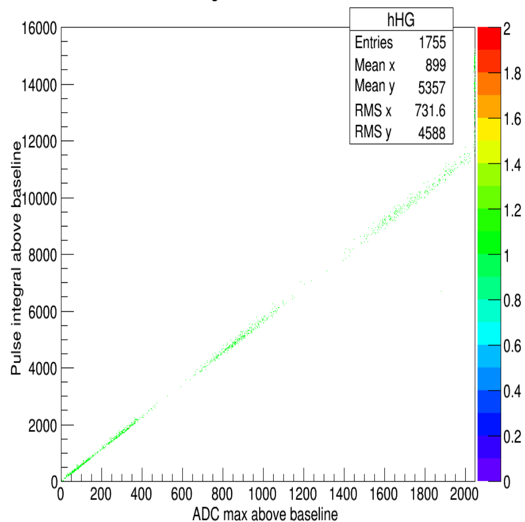
High Gain ADC Data
