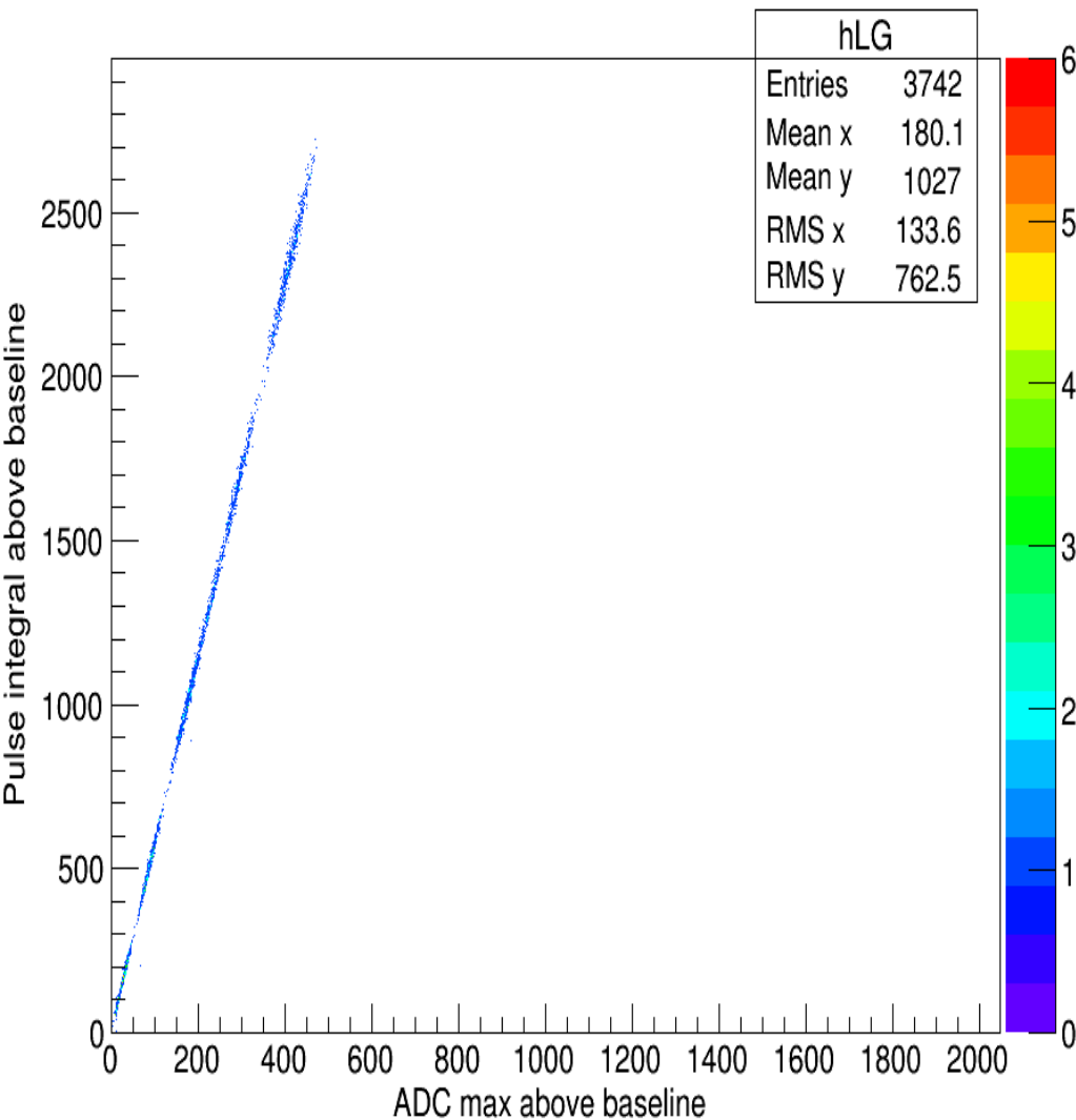
Low Gain ADC Data
