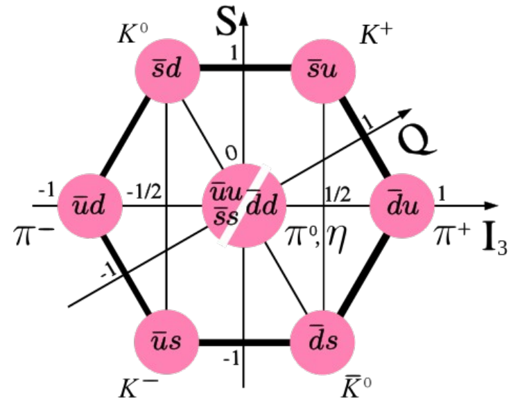
Meson Nonet
