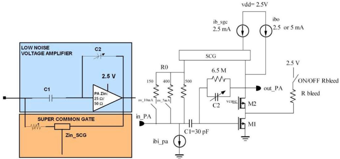
Figure 3 Preamplifier schematic
