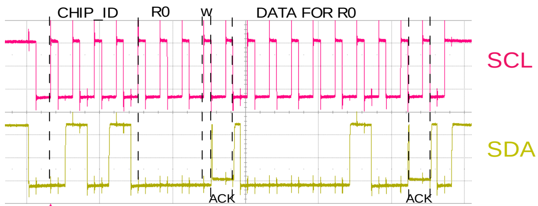
Figure 15 : ZOOM on the Register R0
