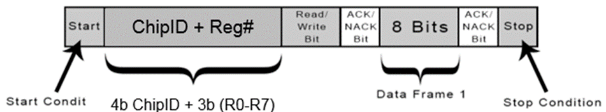
Figure 9 : I2C frame
