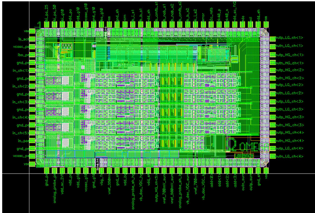
Figure 7: Layout of LAUROC2 (size 3.2 mm x 2 mm)
