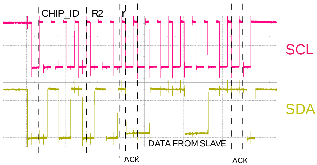
Figure 23 : ZOOM on the Register R2
