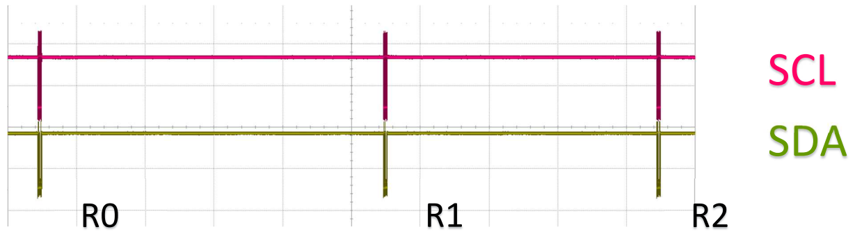
Figure 14 LAUROC2 I2C frame WRITE. Oscilloscope signals.
