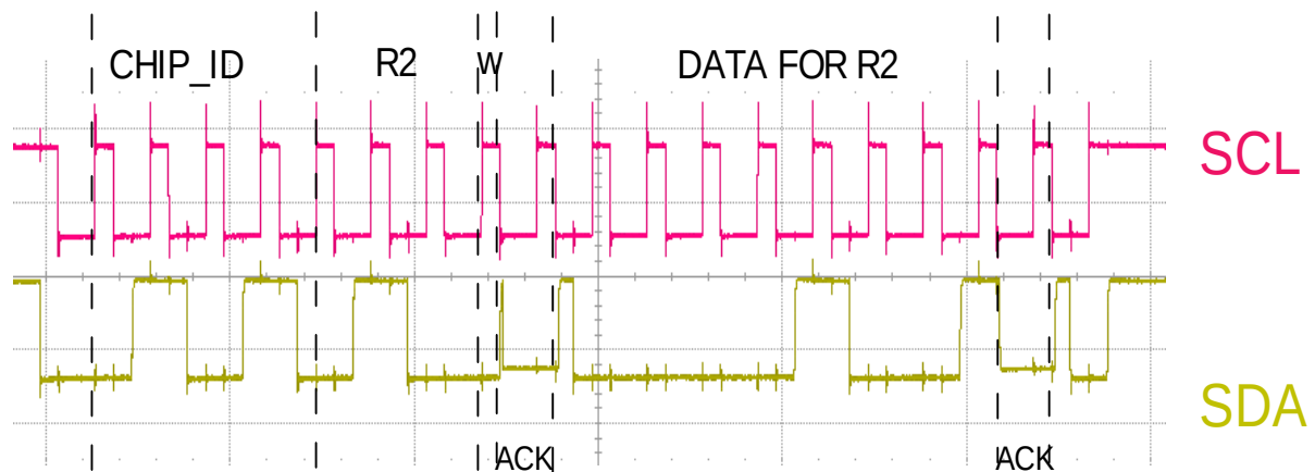
Figure 17 : ZOOM on the Register R2
