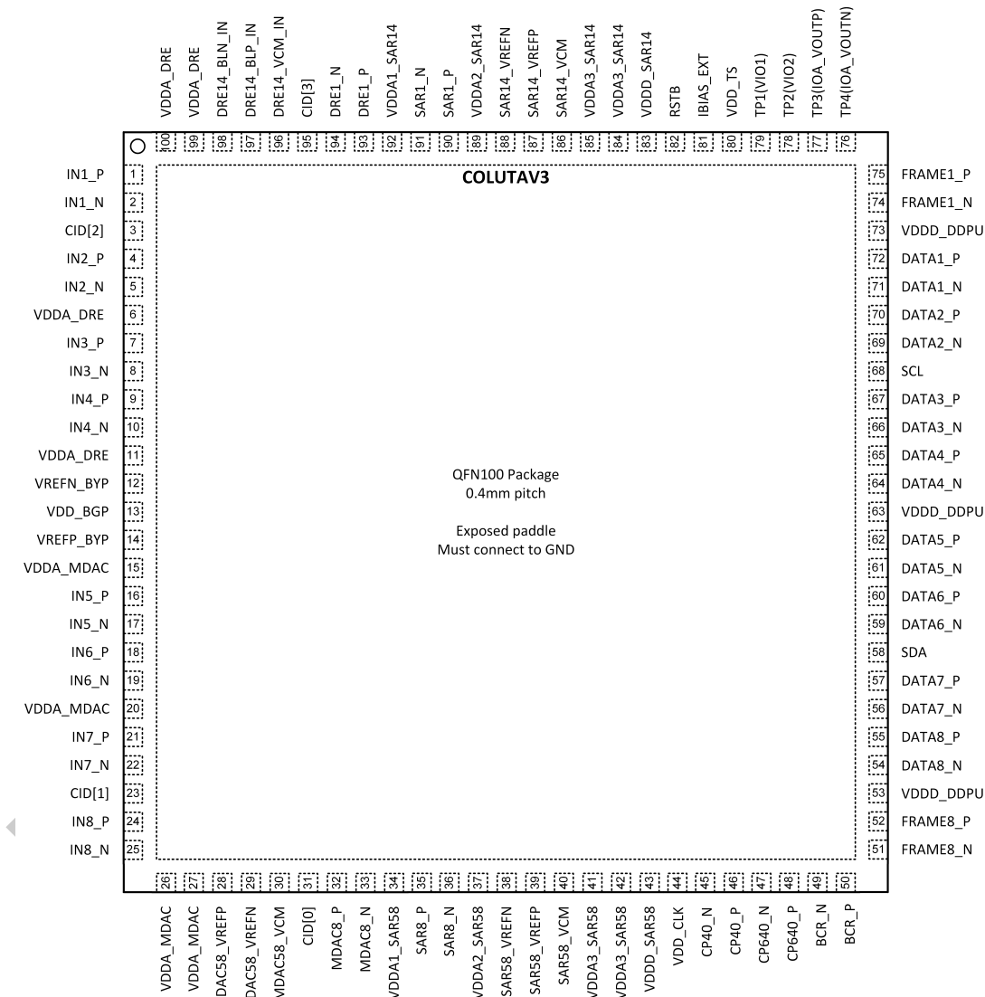
Figure 4: COLUTAV3 pin diagram
